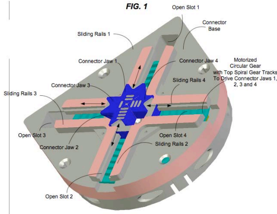
Figure 2: The SINGO connection mechanism.
