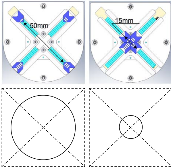
Figure 3: The prototyped dimension of the SINGO connector and the abstract diagrams representing the open and closed state of the connector.
